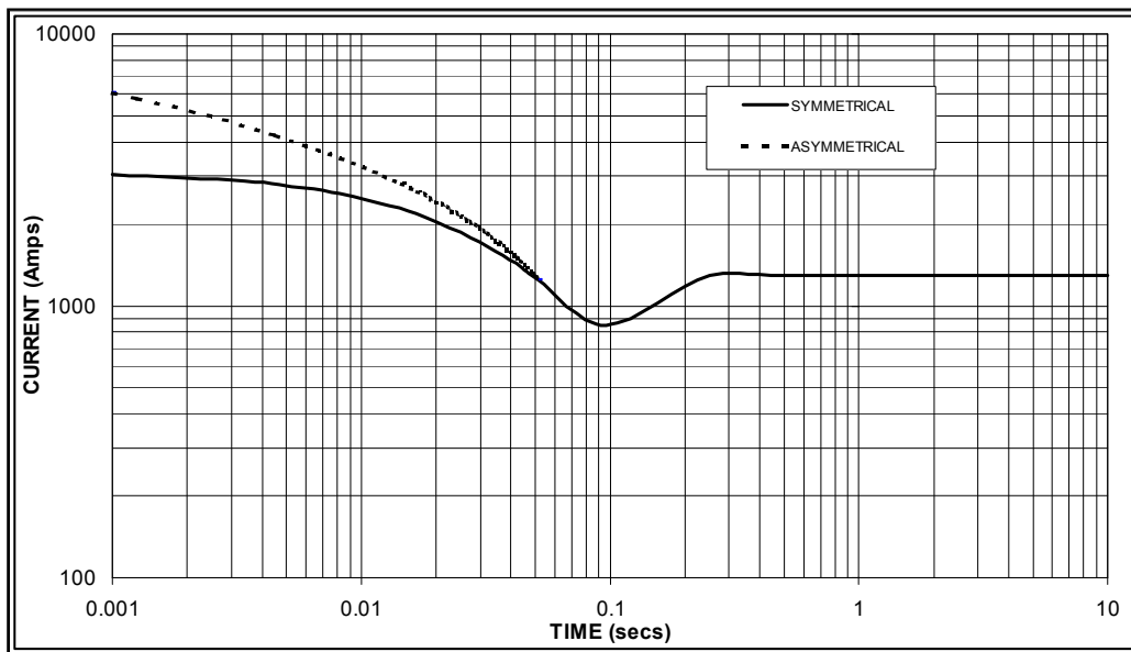
Sustained Short Circuit = 1,200 Amps
